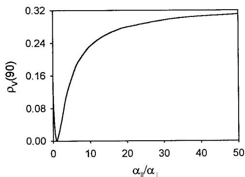
FIGURE 5 Variation of \rho_v(90) with \alpha_{||}/\alpha_{\perp} . The limiting value of \rho_v(90) = 1/3 is only reached for \alpha_{||}/\alpha_{\perp} > 1000 .
