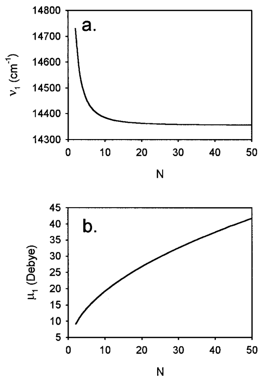
FIGURE 2 Dependence of (a) \tilde{\nu}_1 and (b) \mu_1 on aggregate size N . Parameters used in the calculation are \tilde{\nu}_{\text{mon}} = 15,106 cm -1 , \mu_{\text{mon}} = 6.5 Debye, \beta = 400 cm -1 .
