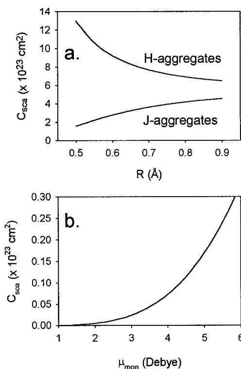
FIGURE 4 (a) Dependence of C_{\text{sca}} at the resonance frequency \tilde{\nu}_1 on the interchromophore distance R in J- and H-aggregates ( N = 100 , \mu_{\text{mon}} = 6.5 Debye). (b) Dependence of C_{\text{sca}} at the resonance frequency \tilde{\nu}_1 on \mu_{\text{mon}} ( N = 100 , R = 0.86 \text{ nm} ) in a J-aggregate. All other parameters are as in Figs. 2 and 3.
